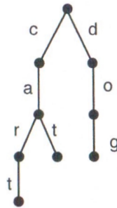
Figure 9.1: Trie
