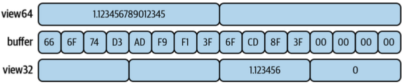
Figure 4-1. Single ArrayBuffer and multiple TypedArray views
