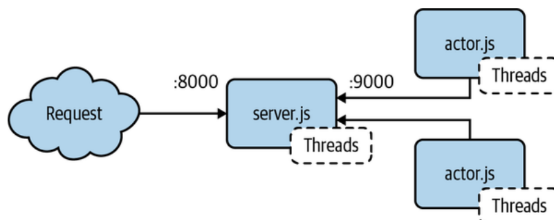
Figure 6-3. A visualization of the actor model implementation in this section
